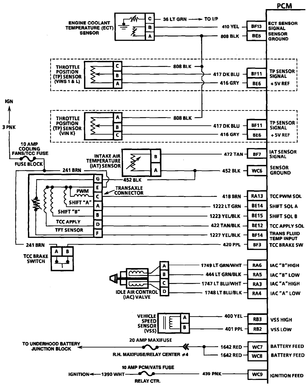
Powertrain Control Module (PCM) 2 Of 5
