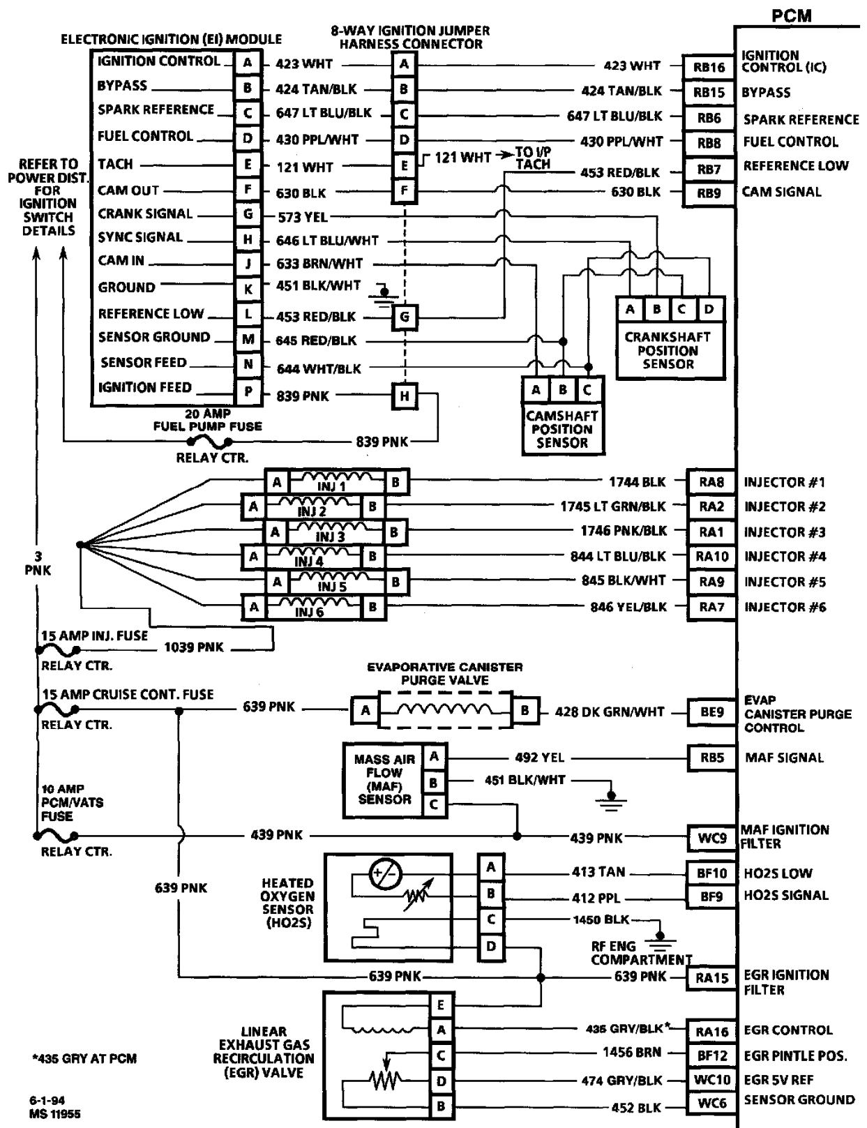
Powertrain Control Module (PCM) Wiring Diagram 1 Of 5
