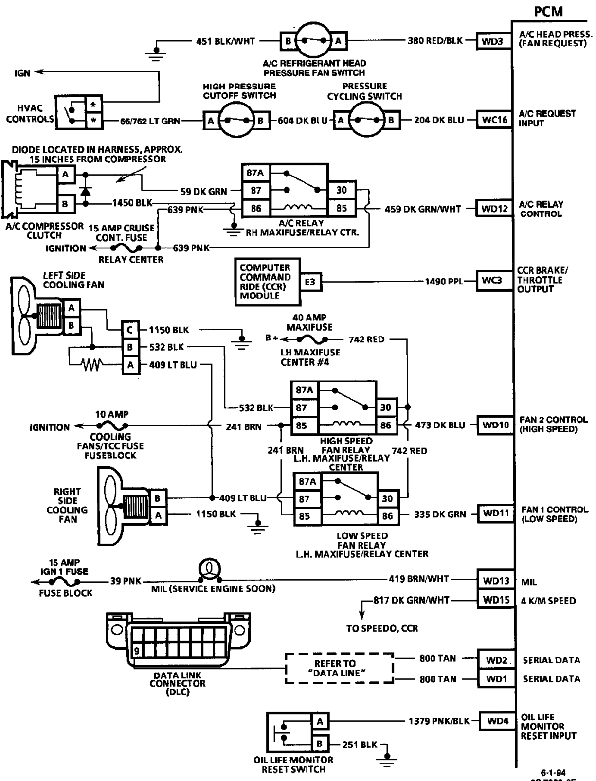
Powertrain Control Module (PCM) Wiring Diagram 4 Of 5
