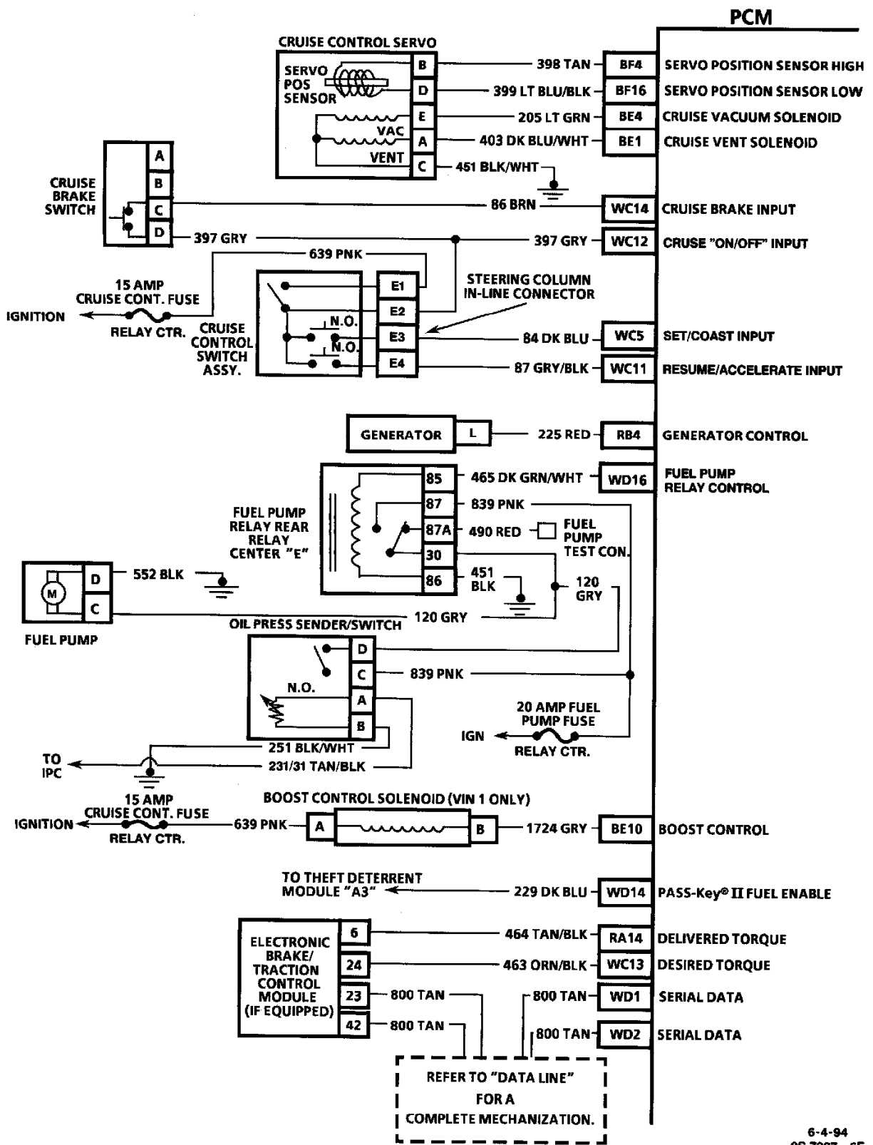
Powertrain Control Module (PCM) Wiring Diagram 3 Of 5
