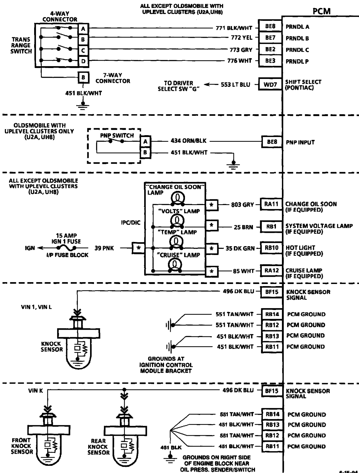
Powertrain Control Module (PCM) Wiring Diagram 5 Of 5
